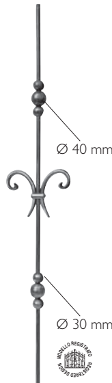
Art. 1064/4 Ø 12 mm H 1000 mm L 180 mm
