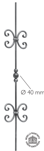
Art. 1064/2 Ø 12 mm H 1000 mm L 175 mm
